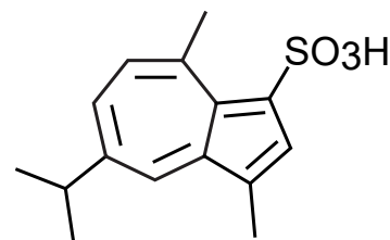
5-propyl-3,8-dimethyl- 1-azulenesulfonic acid (gualenic acid)
